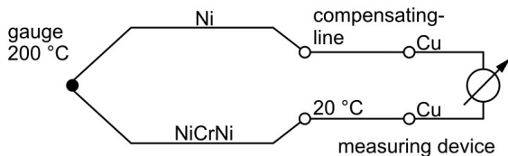
Without-Inert metal-Thermocouple
